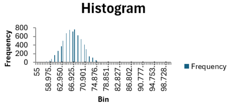
Figure 1 : The histogram shows exam scores concentrated between 62 and 70, with the highest frequency at bin 66.925, confirming a near-normal distribution centred around the mean of 67.24.
